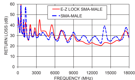
QBL6SMQ-SM+ RETURN LOSS
