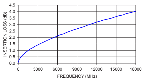
QBL6SMQ-SM+ INSERTION LOSS
