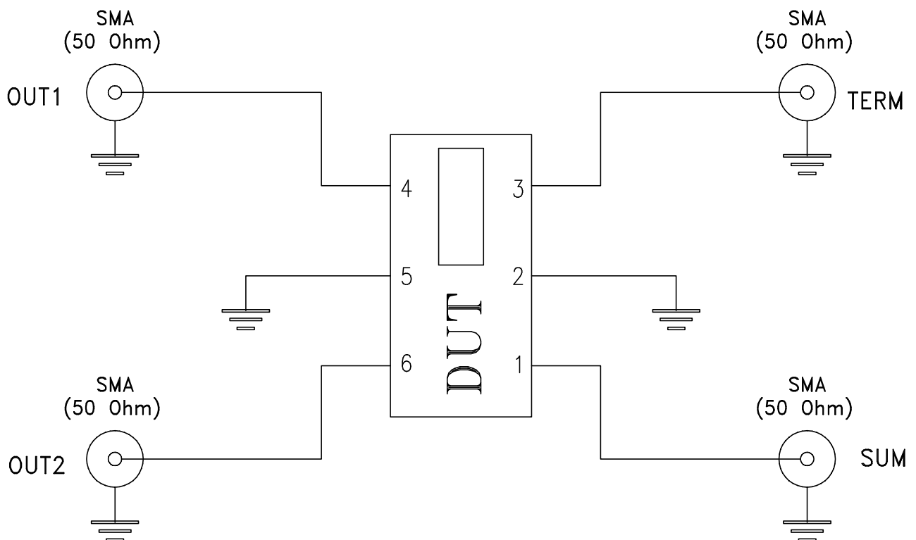
Schematic Diagram
