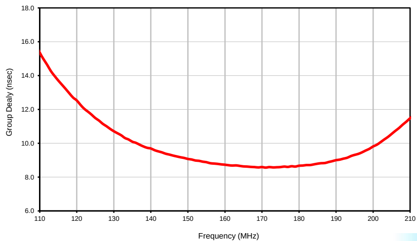
Group Delay
