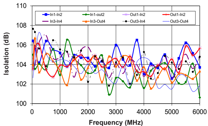
Isolation between channels vs. Frequency
