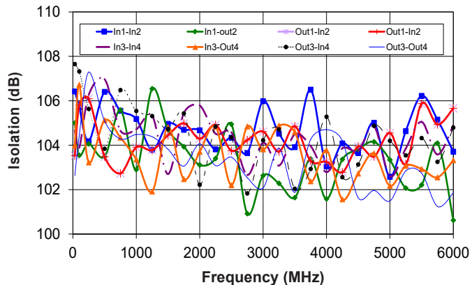
Isolation between channels vs. Frequency
