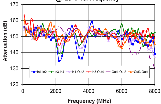
Isolation between channels @+25°C vs. Frequency
