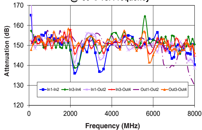
Isolation between channels @+50°C vs. Frequency
