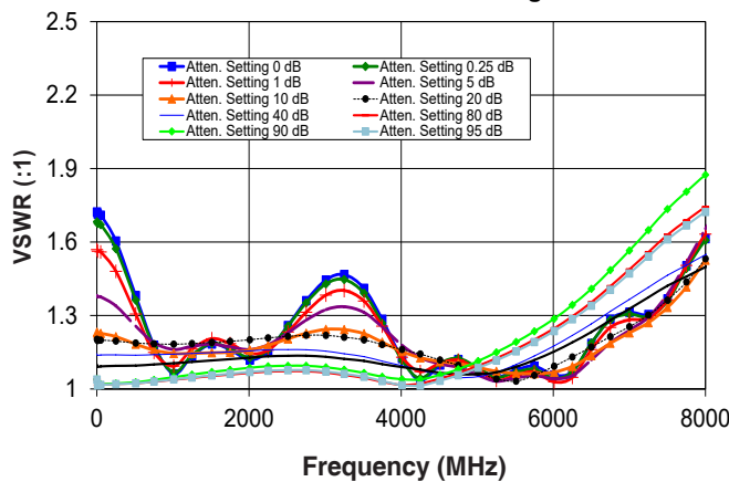
Input VSWR vs. Frequency over Attenuation settings
