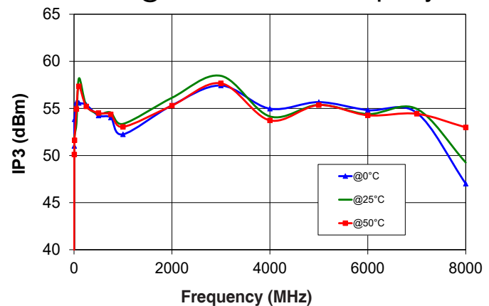
IP3 @ 0dB Attenuation vs. Frequency
