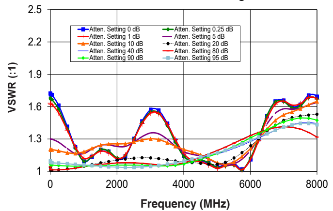
Output VSWR vs. Frequency over Attenuation settings
