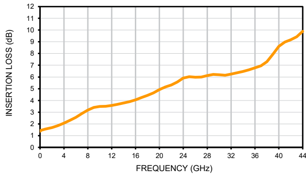
INSERTION LOSS
