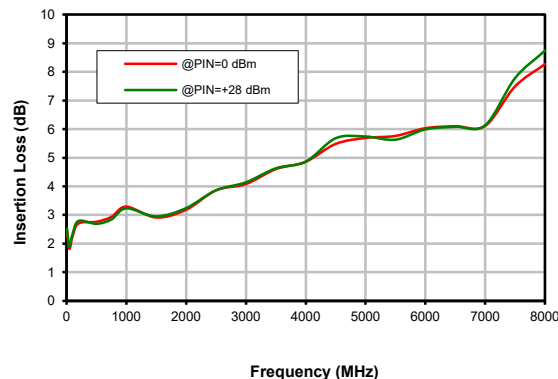
Insertion Loss
