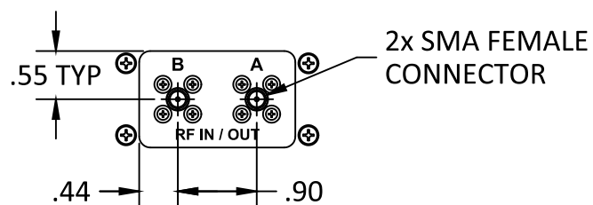
REAR PANEL
