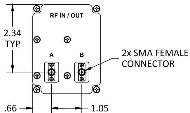
FRONT PANEL
