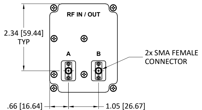
FRONT PANEL
