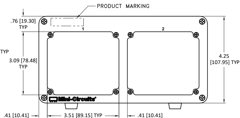
FRONT PANEL FOR RCM WITH SP8T SWITCHES
