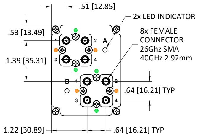
DUAL MTS 26GHz DUAL MTS 40GHz
