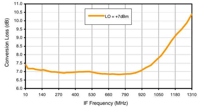
Conversion Loss vs. IF @ RF=3010.1MHz
