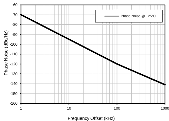
Phase Noise
