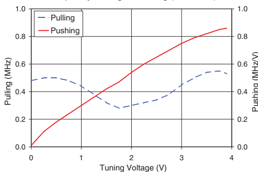
ROS-1590-319+ Frequency Pulling & Pushing (Vcc ± 5%)
