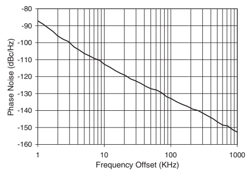
ROS-1590-319+ Phase Noise
