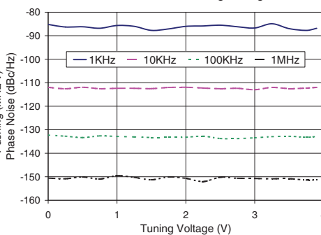
ROS-1590-319+ Phase Noise Vs. Tuning Voltage
