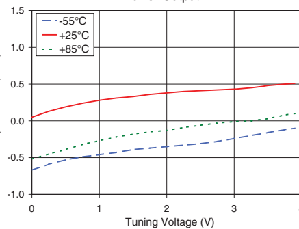
ROS-1590-319+ Power Output
