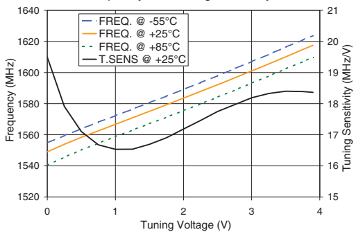
ROS-1590-319+ Frequency and Tuning Sensitivity
