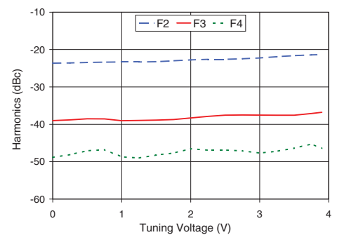
ROS-1590-319+ Harmonics Level
