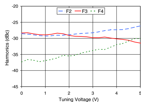
ROS-1850-519+ Harmonics Level
