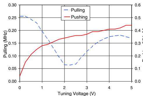
ROS-1850-519+ Frequency Pulling & Pushing (Vcc ± 5%)
