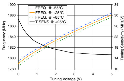
ROS-1850-519+ Frequency and Tuning Sensitivity
