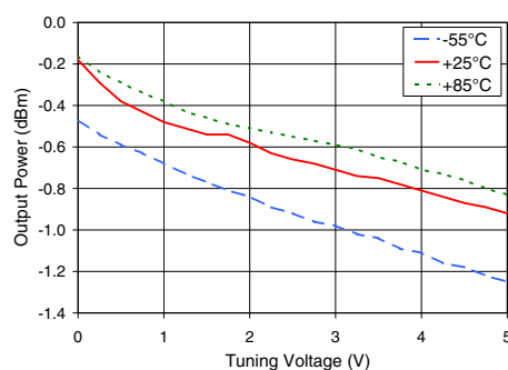
ROS-1850-519+ Power Output
