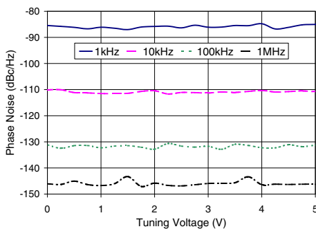
ROS-1850-519+ Phase Noise Vs. Tuning Voltage
