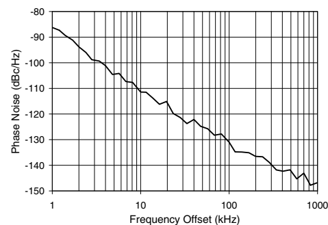
ROS-1850-519+ Phase Noise
