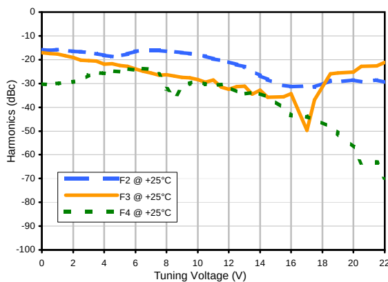
Harmonics Level
