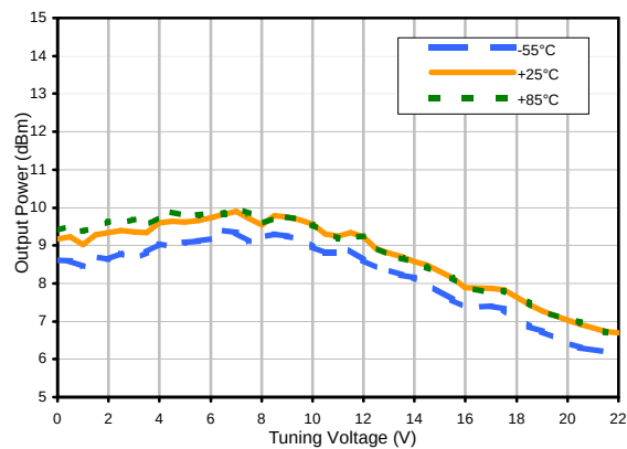
Power Output
