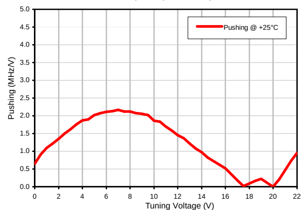
Frequency Pushing
