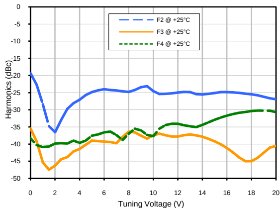
Harmonics Level
