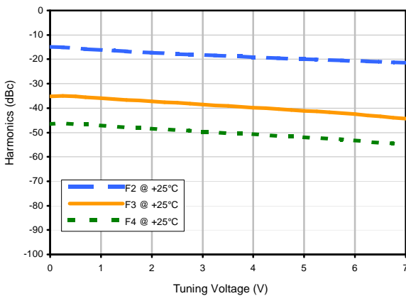
Harmonics Level
