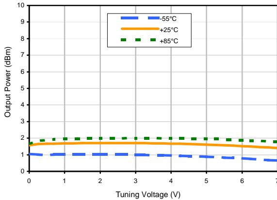
Power Output
