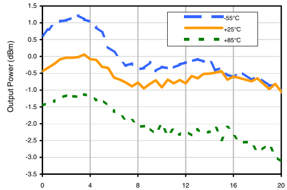
Power Output
