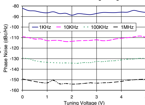
ROS-638+ Phase Noise Vs. Tuning Voltage
