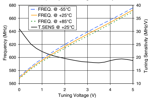
ROS-638+ Frequency and Tuning Sensitivity
