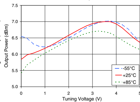
ROS-638+ Power Output
