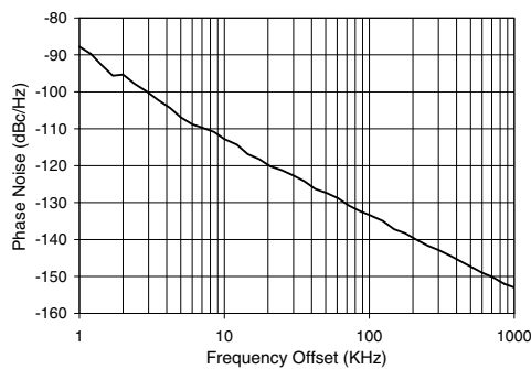
ROS-638+ Phase Noise
