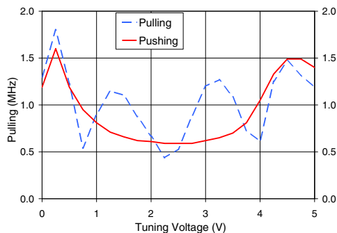
ROS-638+ Frequency Pulling & Pushing (Vcc ± 5%)
