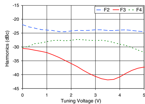
ROS-638+ Harmonics Level
