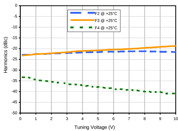
Harmonics Level
