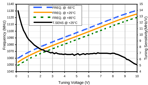
Frequency and Tuning Sensitivity
