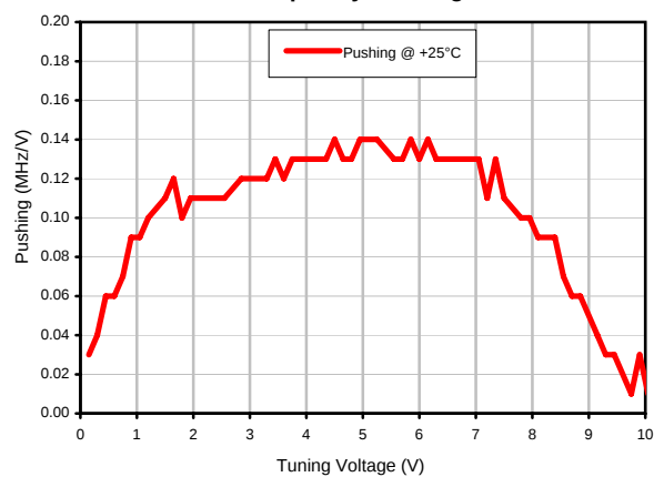
Frequency Pushing
