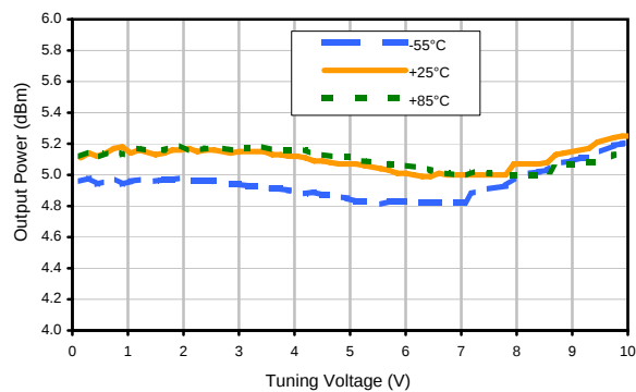
Power Output
