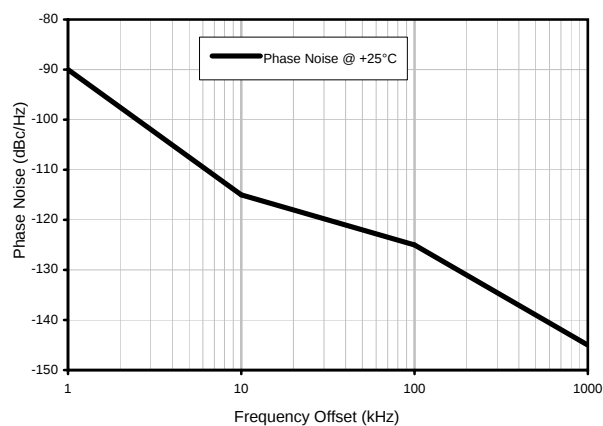
Phase Noise
