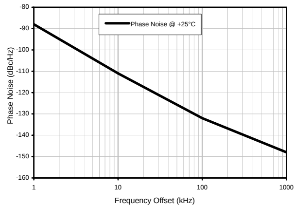
Phase Noise
