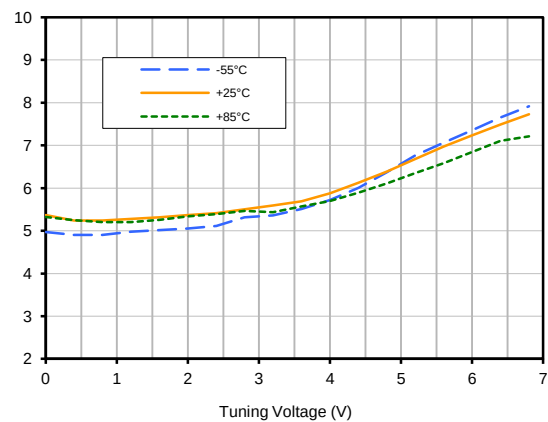
Output Power
