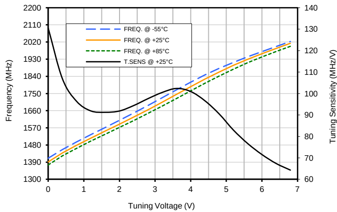
Frequency and Tuning Sensitivity
