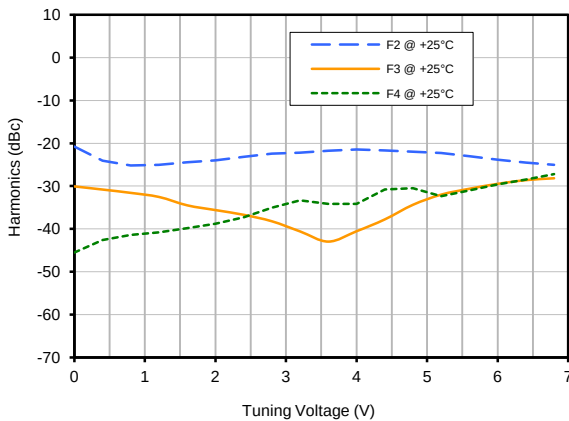
Harmonics Level
