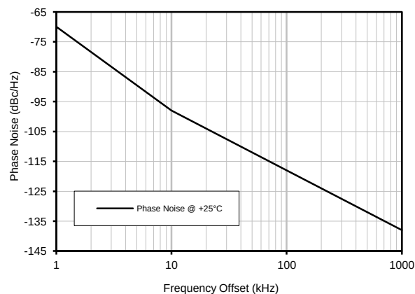
Phase Noise
