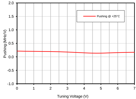
Frequency Pushing
