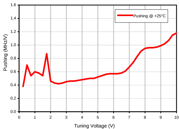
Frequency Pushing
