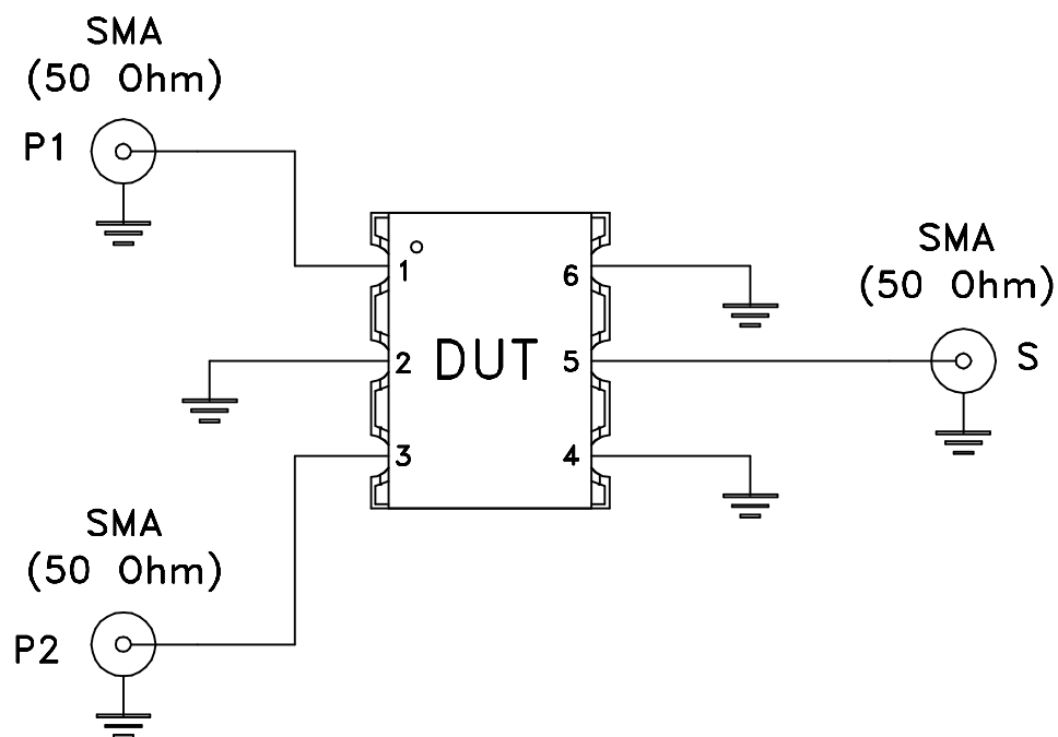
Schematic Diagram
