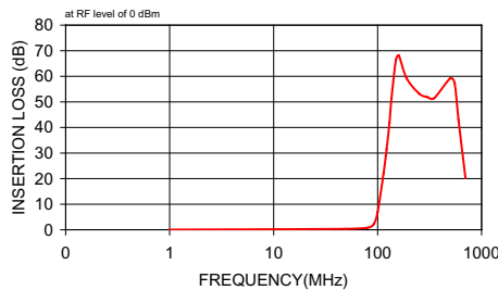
SALF-78 INSERTION LOSS
