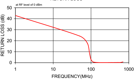
SALF-78 RETURN LOSS
