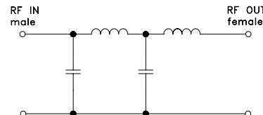
electrical schematic
