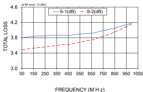
TOTAL LOSS
