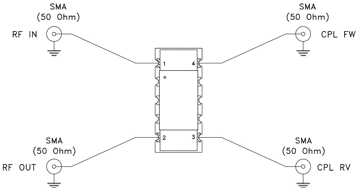
Schematic Diagram
