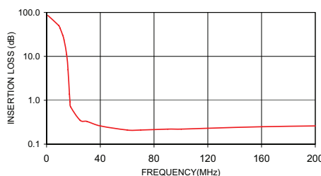
SCHF-17 INSERTION LOSS
