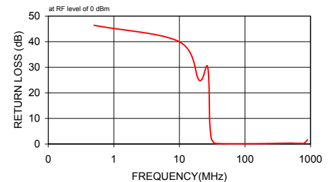
SCLF-27 RETURN LOSS
