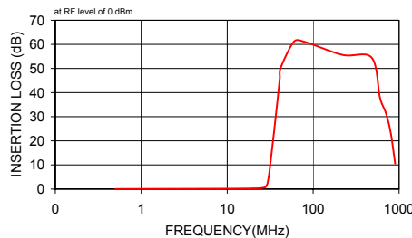
SCLF-27 INSERTION LOSS
