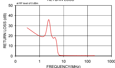
SCLF-5 RETURN LOSS
