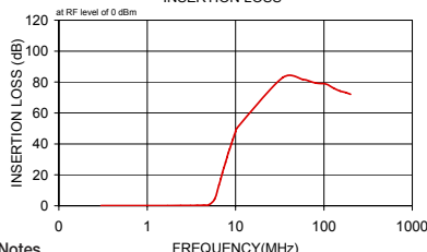
SCLF-5 INSERTION LOSS
