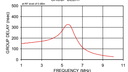
SCLF-5 GROUP DELAY
