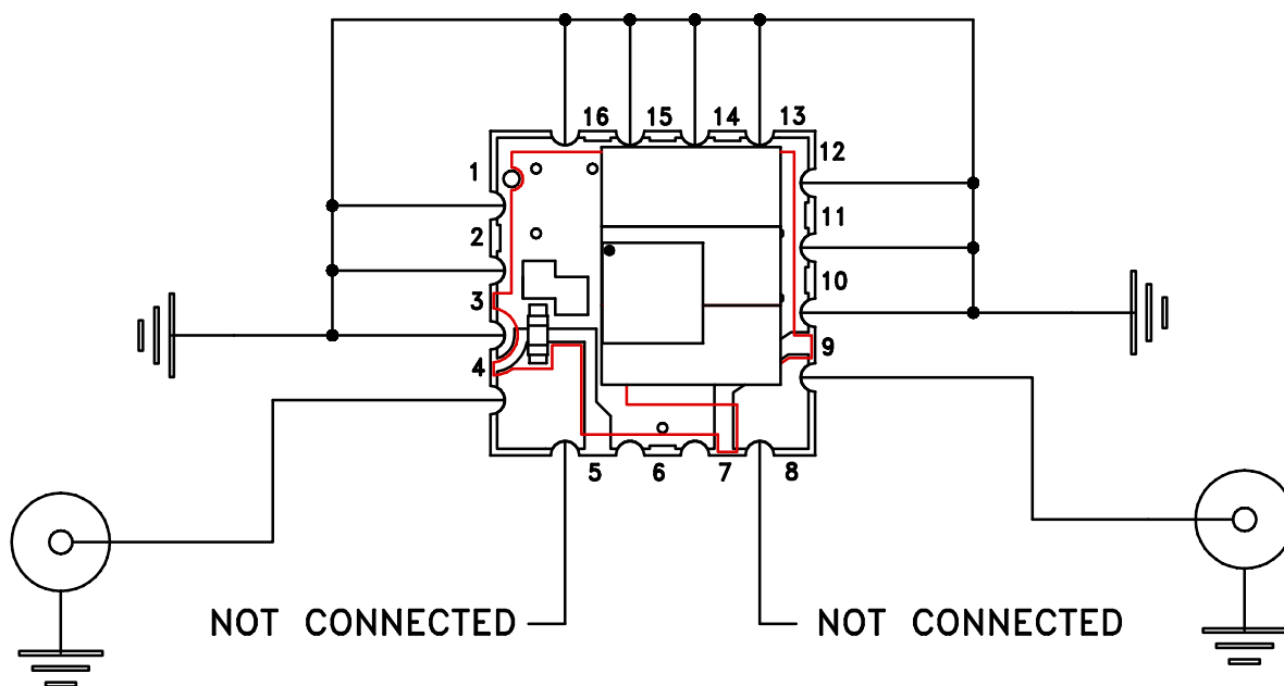
Schematic Diagram
