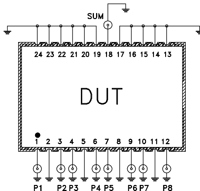
Schematic Diagram
