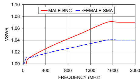
SF-BM-6 VSWR
