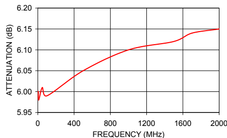
SF-BM-6 ATTENUATION
