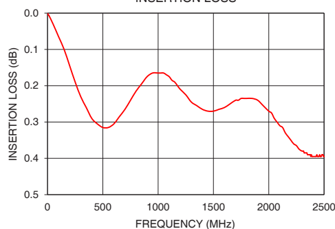
SFMP-5075+ INSERTION LOSS
