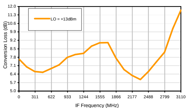
Conversion Loss vs. IF @ RF=7210.1001MHz
