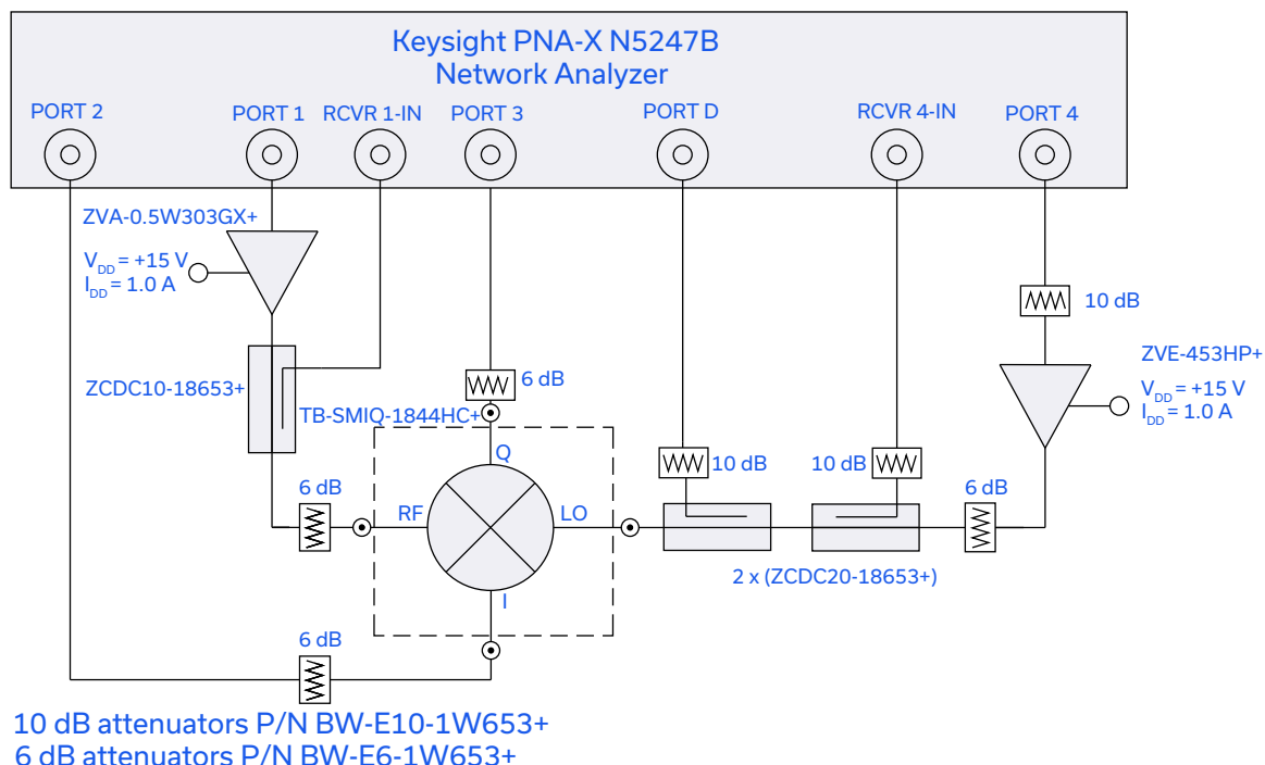
Figure 5. Block diagram of test circuit used to characterize Compression
