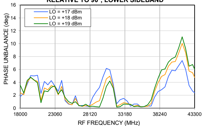
PHASE UNBALANCE @ FIXED IF = 200 MHz RELATIVE TO 90°, LOWER SIDEBAND
