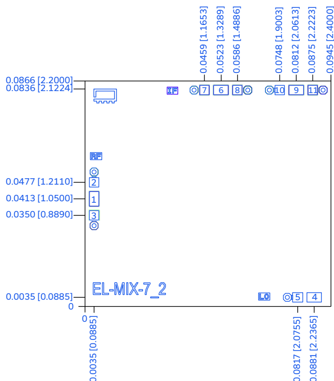
Figure 2: SMIQ-1844H-D+ Die Outline.
