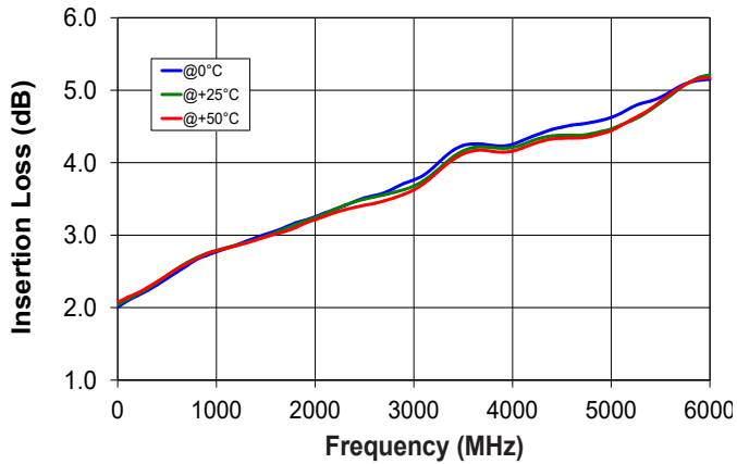
Insertion Loss over Temperature
