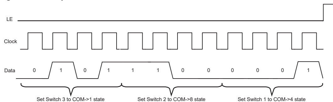
Figure 4: Example of command for 3 switches in series
