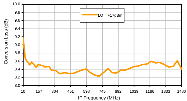
Conversion Loss vs. IF @ RF=1500.1MHz
