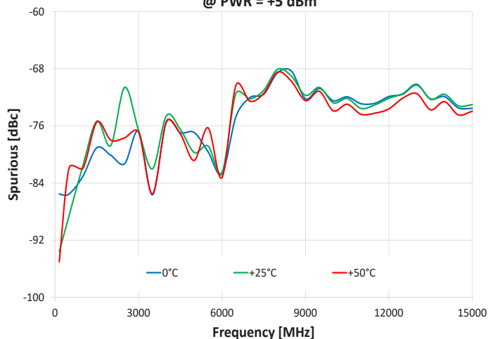
Spurious @ \pm 100 kHz to 50 MHz offset vs. Frequency @ PWR = +5 dBm
