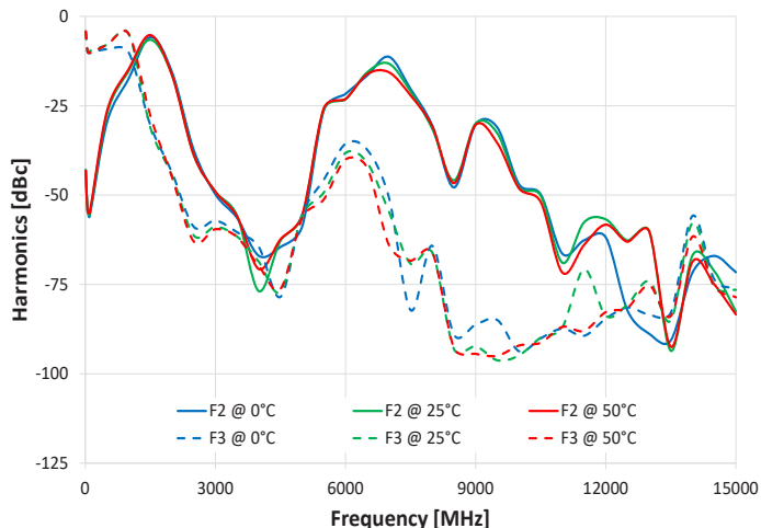
Harmonics vs. Frequency @ PWR = +10 dBm
