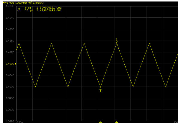
Triangle signal, 1400 - 1415 MHz, 50 \mu s, within sub-bandwidth
