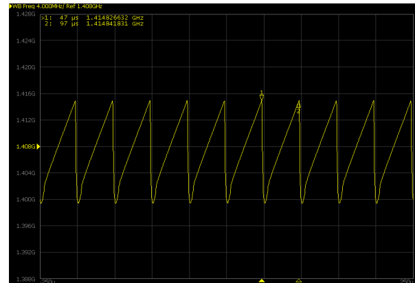
Sawtooth signal, 1400 - 1415 MHz, 50 \mu s, within sub-bandwidth
