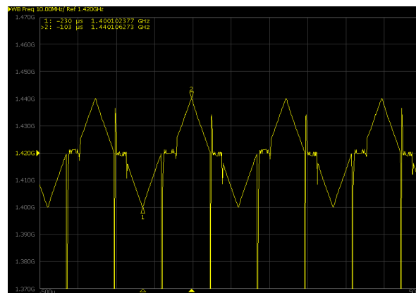
Triangle signal, 1400 - 1440 MHz, 100 \mu s, over sub-bandwidth
