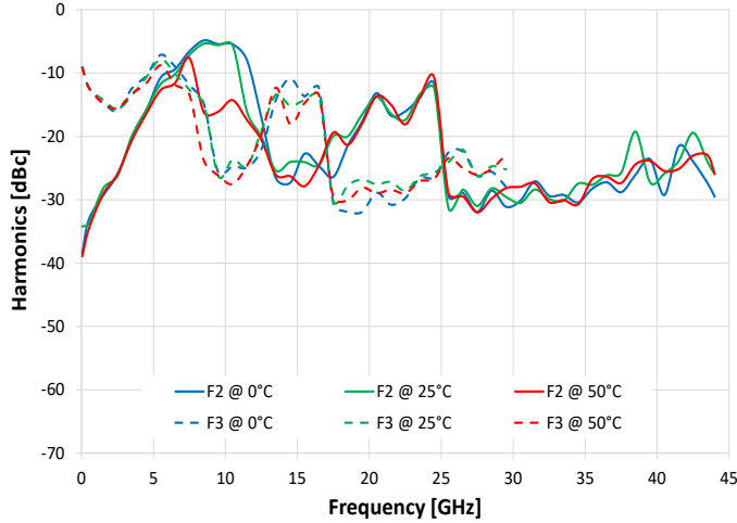
Harmonics vs. Frequency @ -10 dBm
