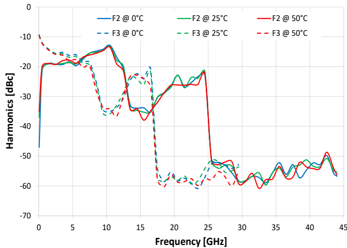
Harmonics vs. Frequency @ 0 dBm
