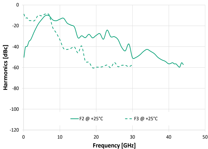
Harmonics vs. Output Frequency @ -10 dBm
