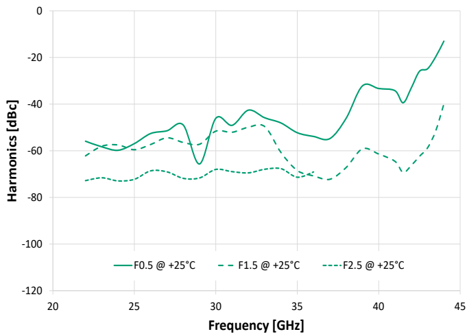
Sub-Harmonics vs. Output Frequency @ 0 dBm
