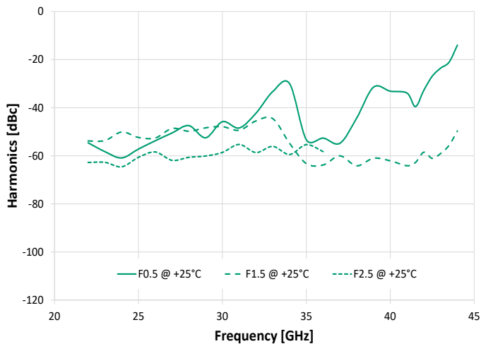
Sub-Harmonics vs. Output Frequency @ -10 dBm
