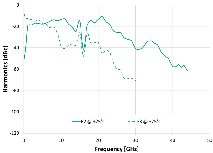
Harmonics vs. Output Frequency @ 0 dBm
