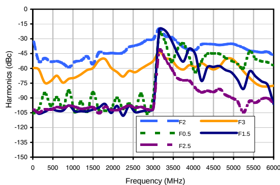
Harmonics & Sub-Harmonics Levels Vs. Output Frequency PWR=+10dBm
