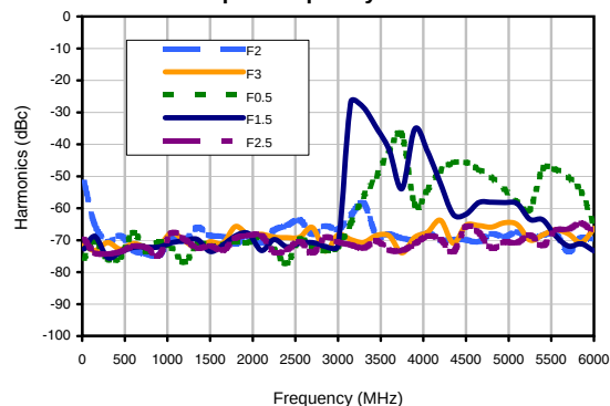
Harmonics & Sub-Harmonics Levels Vs. Output Frequency PWR=-20dBm
