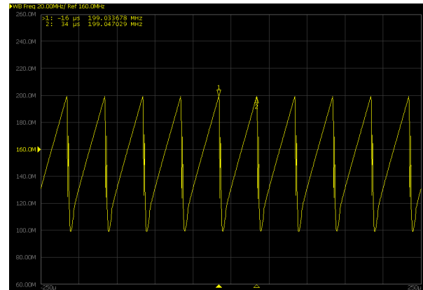
Sawtooth signal, 8300 - 8400 MHz, 50 μs, within sub-bandwidth
